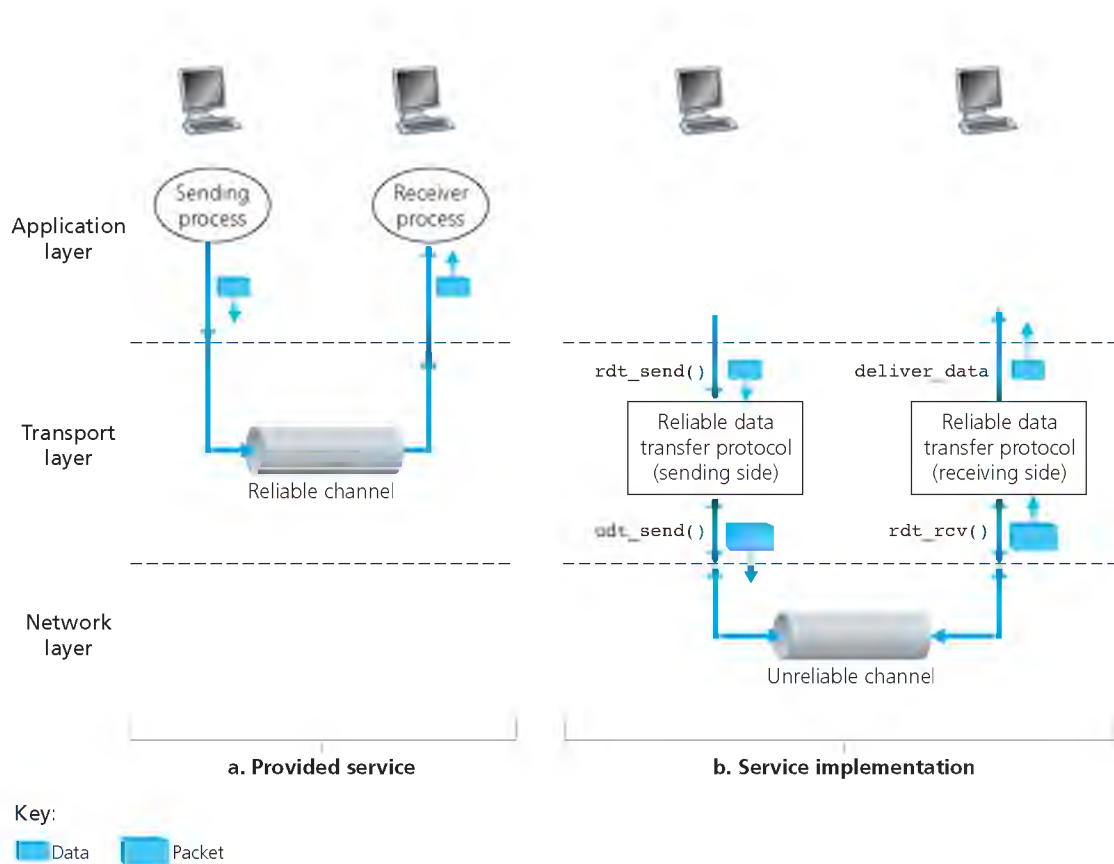
Figure 3.8 ♦ Reliable data transfer: Service model and service implementation
