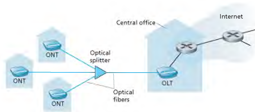
Figure 1.7 ♦ FTTH Internet access
