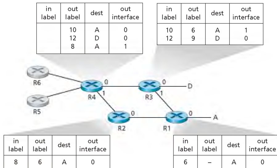
Figure 5.29 ♦ MPLS-enhanced forwarding
