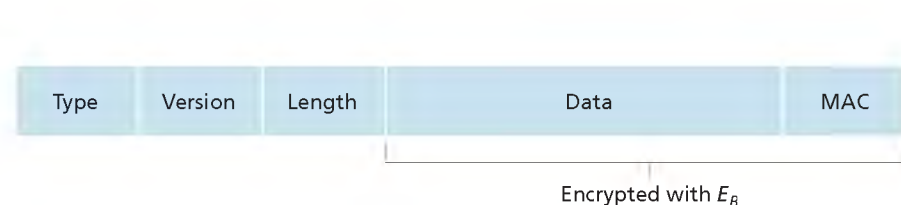
Figure 8.26 ♦ Record format for SSL
