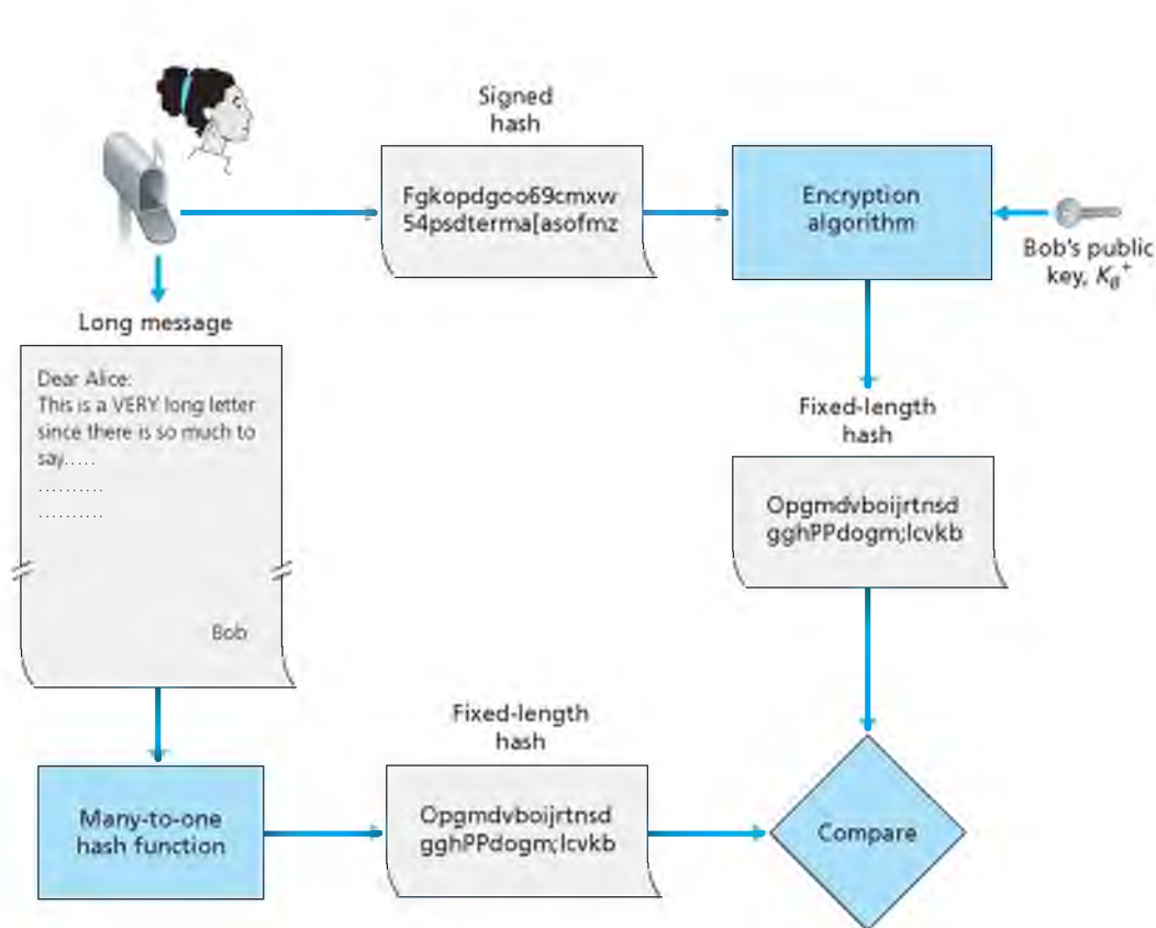
Figure 8.12 ♦ Verifying a signed message
