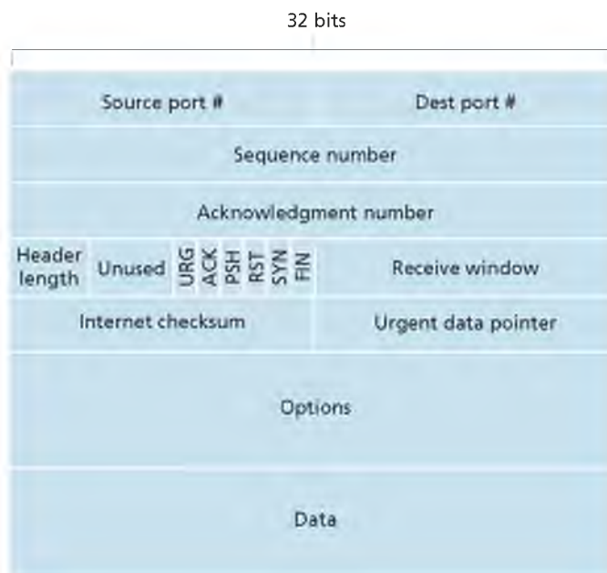
Figure 3.29 ♦ TCP segment structure
