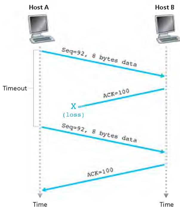
Figure 3.34 ♦ Retransmission due to a lost acknowledgment
