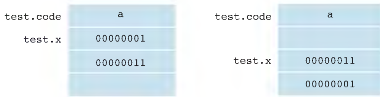
Figure 9.6 ♦ Two different data layouts on two different architectures
