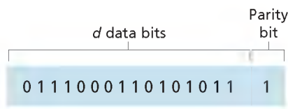
Figure 5.4 ♦ One-bit even parity
