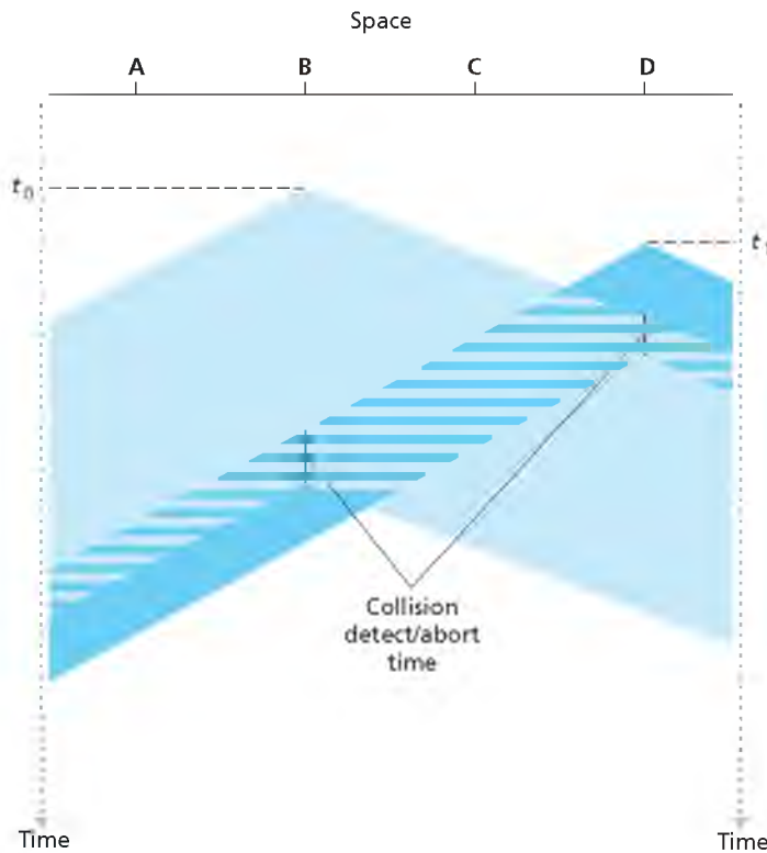
Figure 5.13 ♦ CSMA with collision detection
