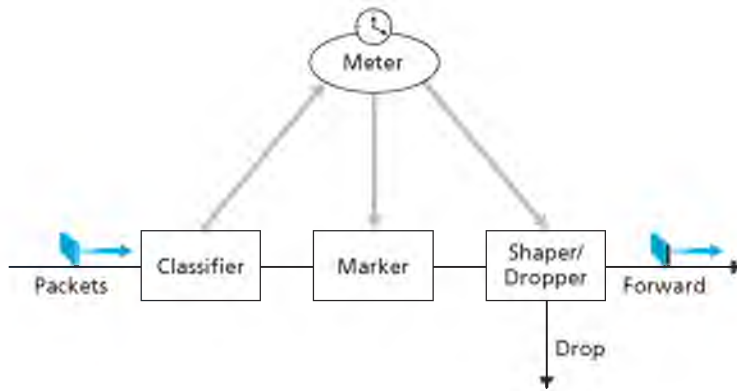
Figure 7.26 ♦ A simple Diffserv network example
