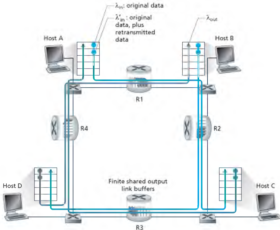
Figure 3.47 ♦ Four senders, routers with finite buffers, and multipath paths
