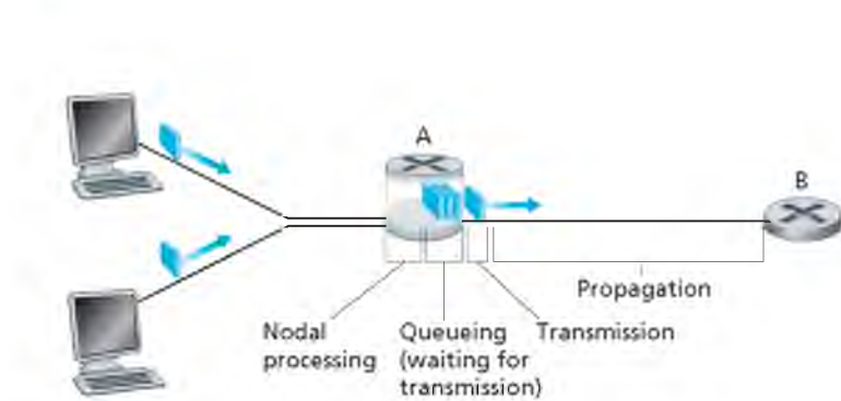
Figure 1.16 ♦ The nodal delay at router A
