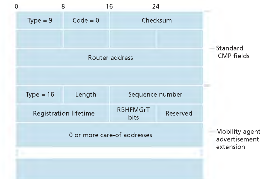
Figure 6.27 ♦ ICMP router discovery message with mobility agent advertisement extension
