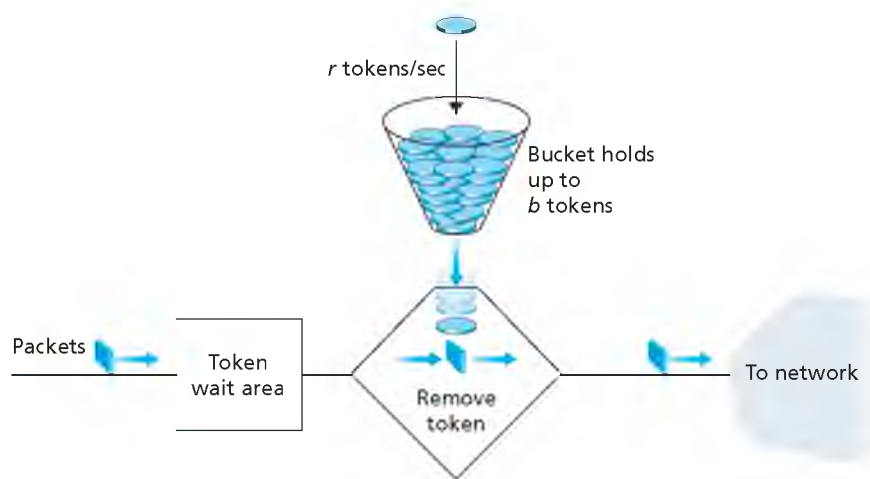
Figure 7.23 ♦ The leaky bucket policer
