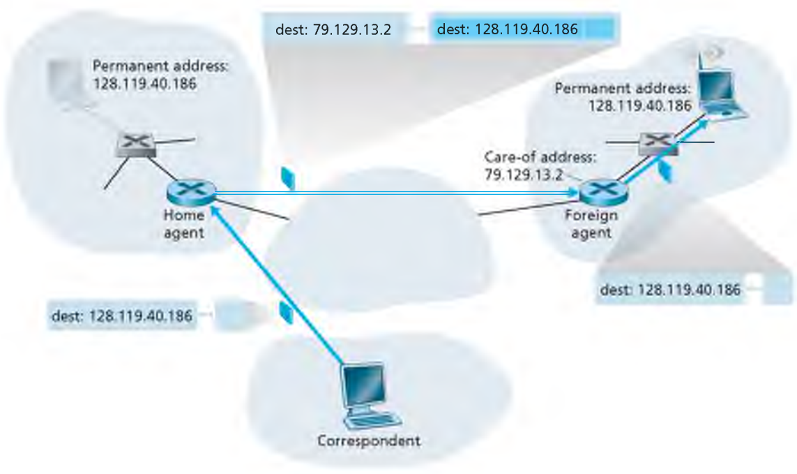
Figure 6.24 ♦ Encapsulation and decapsulation
