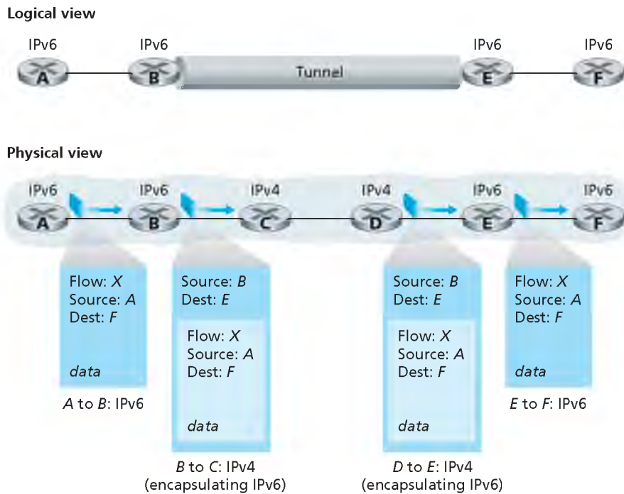
Figure 4.26 ♦ Tunneling
