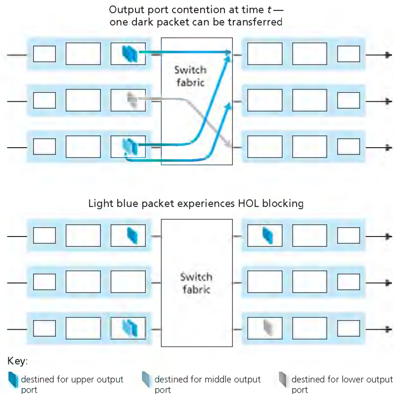
Figure 4.11 ♦ HOL blocking at an input queued switch
