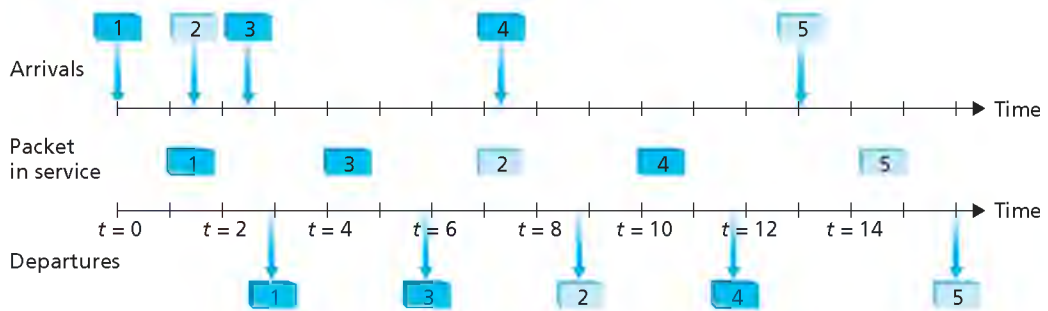
Figure 7.20 ♦ Operation of the priority queue
