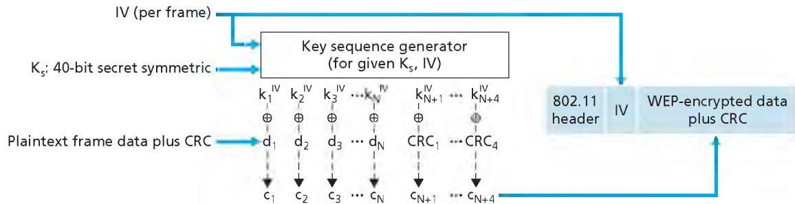
Figure 8.30 ♦ 802.11 WEP protocol
