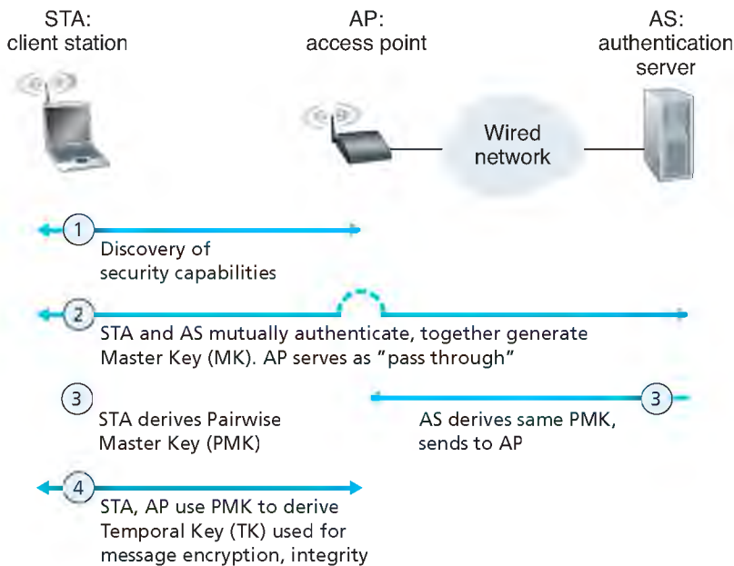
Figure 8.31 ♦ 802.11i: four phases of operation
