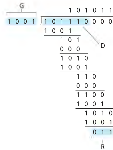
Figure 5.7 ♦ A sample CRC calculation
