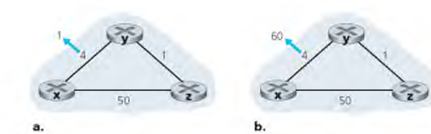
Figure 4.31 ♦ Changes in link cost
