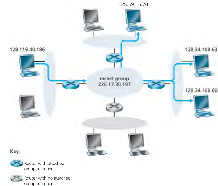
Figure 4.47 ♦ The multicast group: A datagram addressed to the group is delivered to all members of the multicast group
