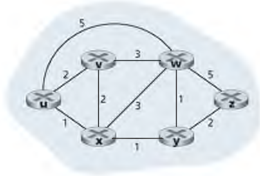
Figure 4.27 ♦ Abstract graph model of a computer network
