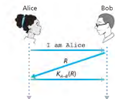
Figure 8.18 ♦ Protocol ap4.0 and a failure scenario
