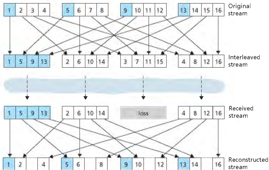
Figure 7.9 ♦ Sending interleaved audio
