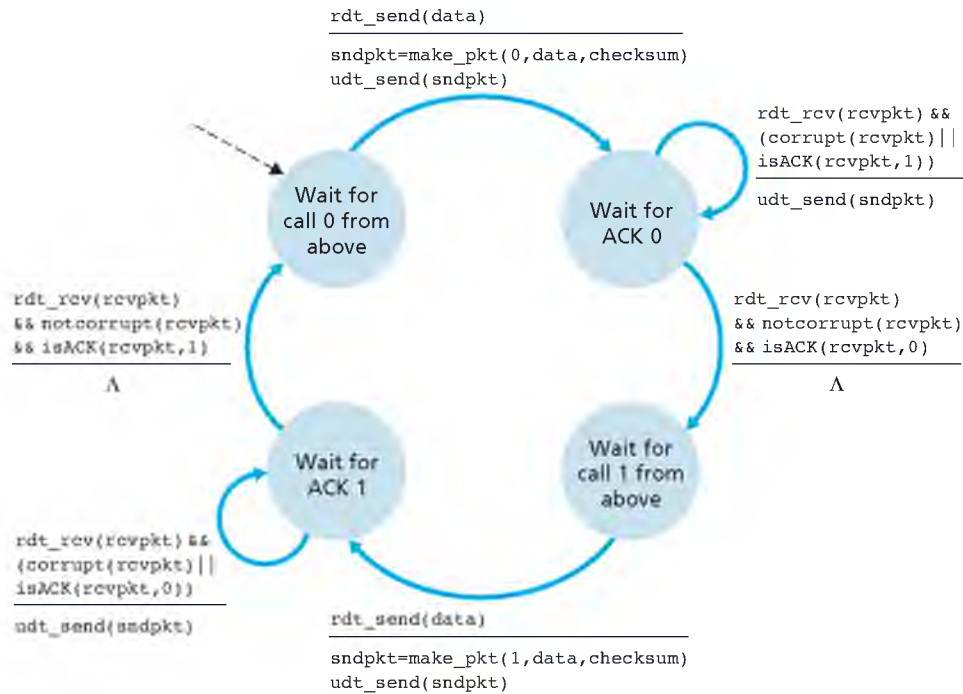
Figure 3.13 ♦ rdt2.2 sender
