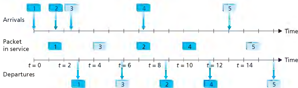
Figure 7.21 ♦ Operation of the two-class round robin queue
